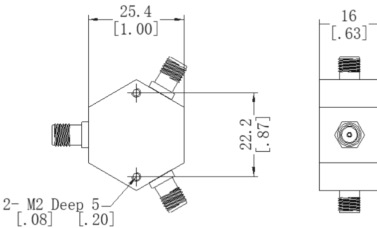
Physical Dimensions (± 0.3mm)
