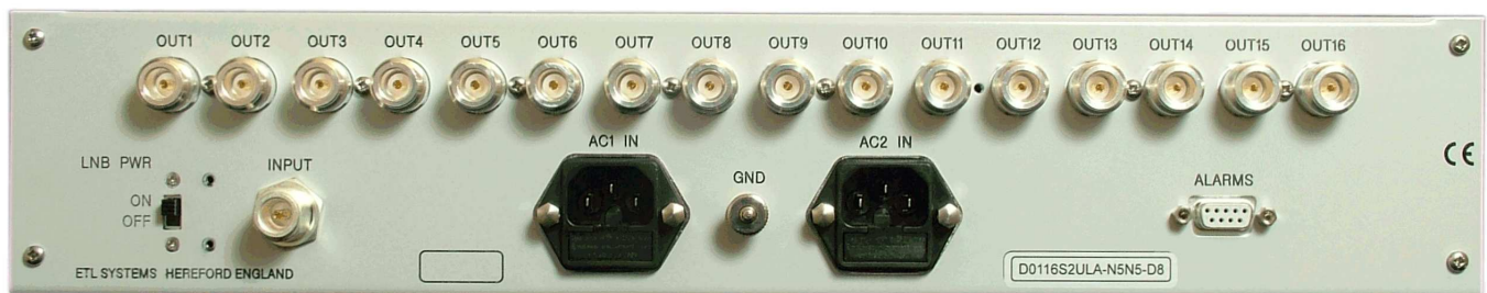
Rear View of Model D0116S2ULA-N5N5-D8 (with 50 ohm N-type connectors)
