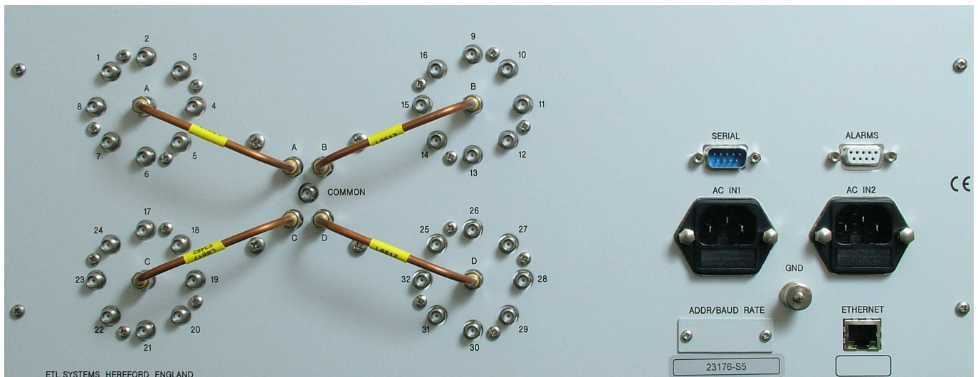
Rear View of Model 23176-S5
