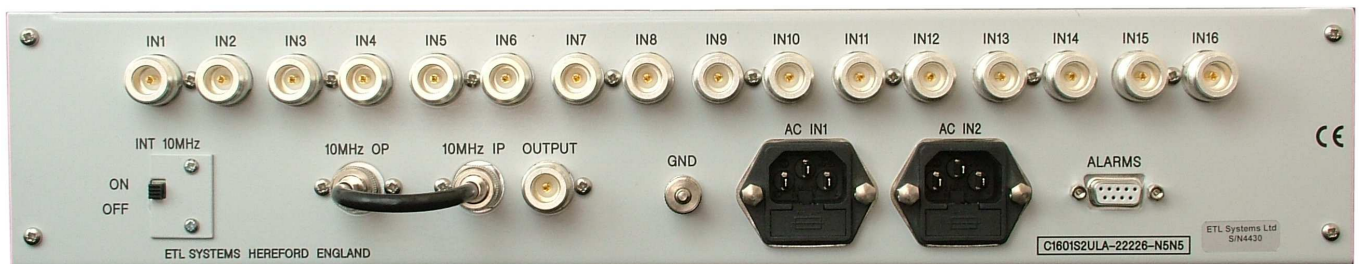
Rear View of Model C1601S1ULA-22226-N5N5
