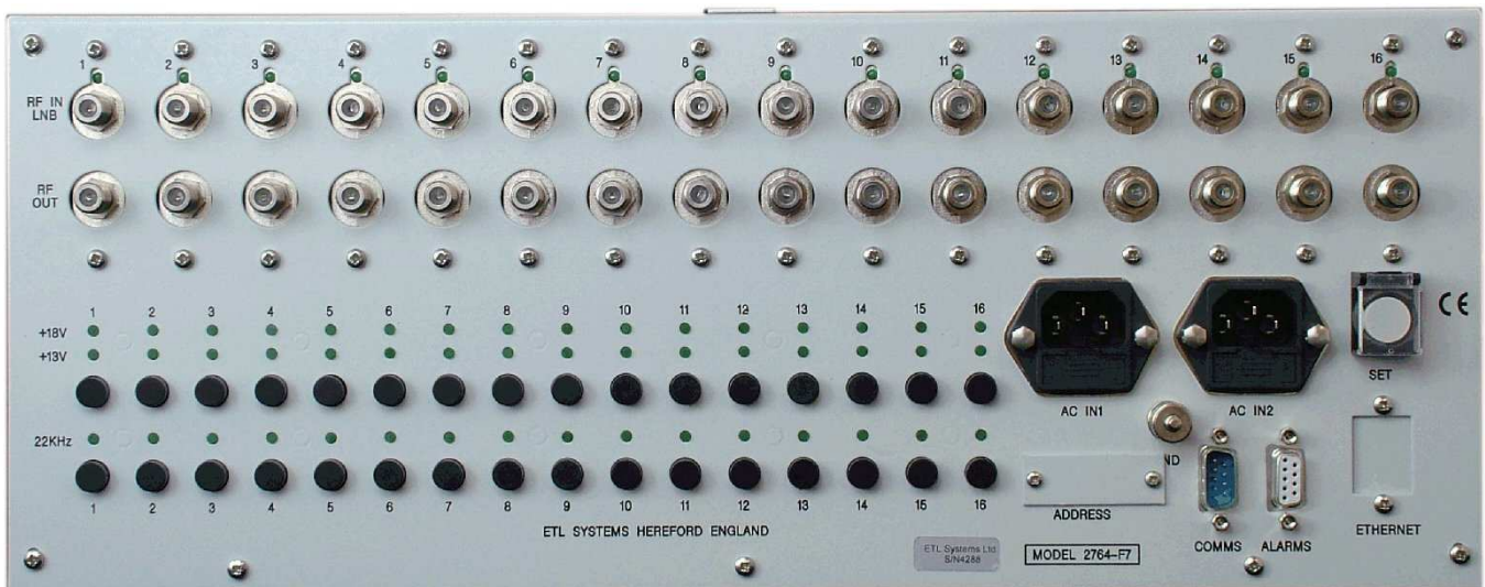
Rear View of Model 2764 with 75 ohm F-type connectors
